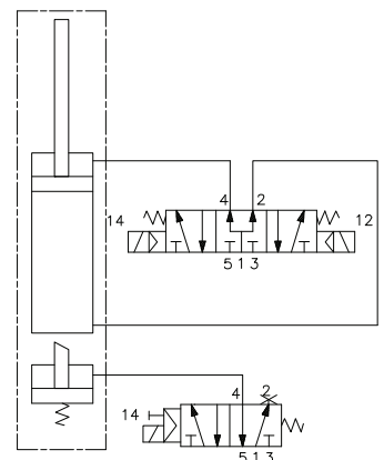
Passive brake
