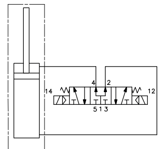
Passive brake
