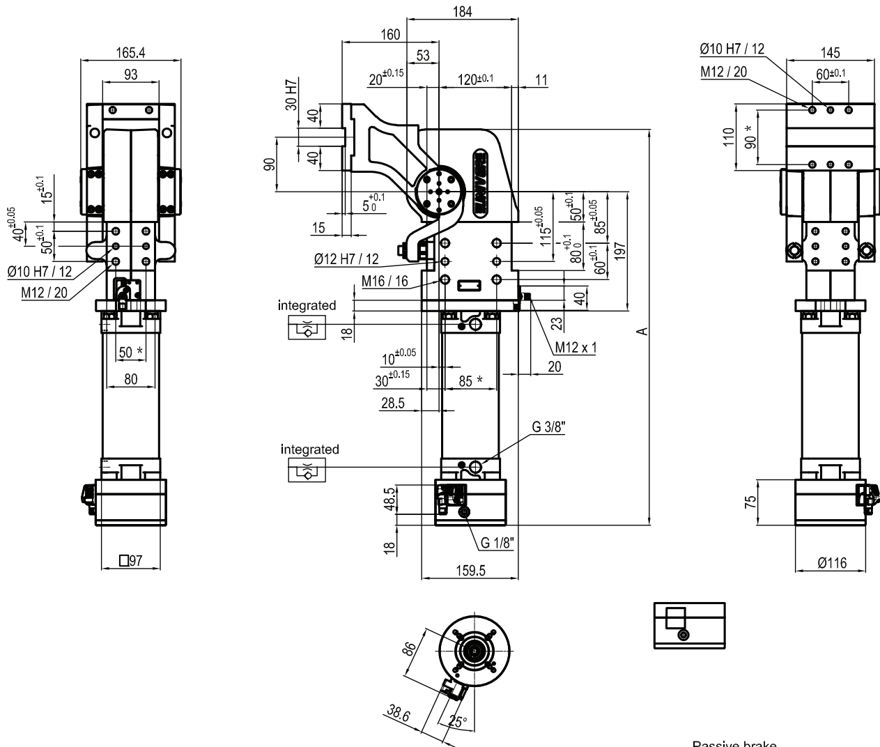
Passive brake
